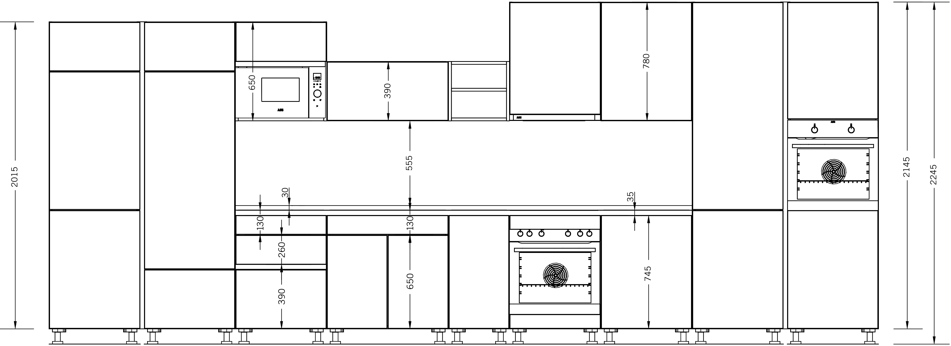
Dimensions in mm
